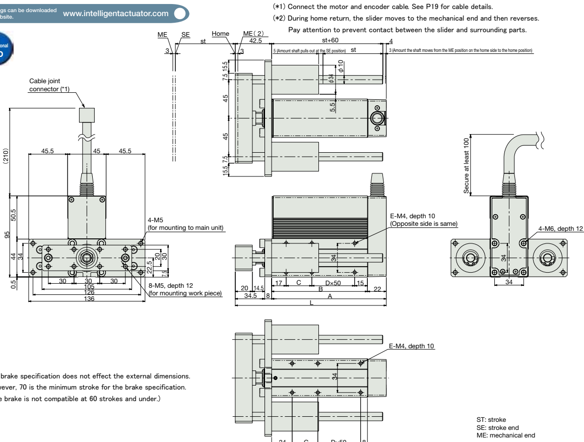
■ Dimensions and Weight by Stroke (If the unit has a brake, add 0.2kg)
