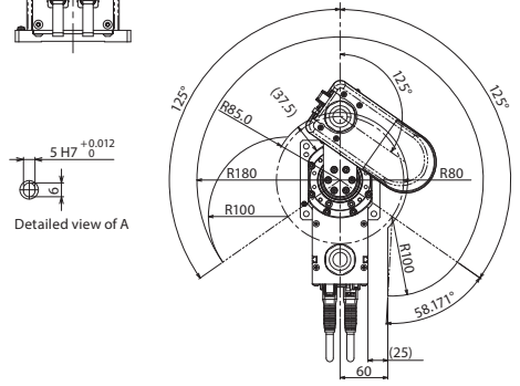
Operation prohibited area Work envelope of the left-arm system
