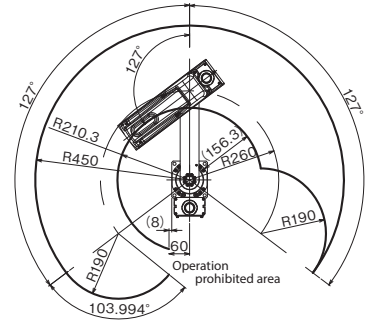
Work envelope of the right-arm system
