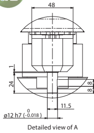
Detailed view of A
