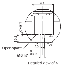
Detailed view of A
