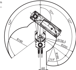
Operation prohibited area Work envelope of the left-arm system
