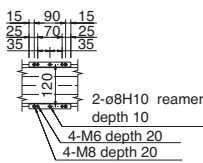
Detail View of Z-Axis slider
