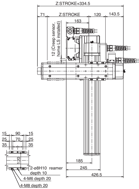
Detail View of Z-Axis slider
