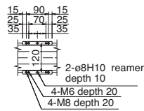
Detail View of Z-Axis slider
