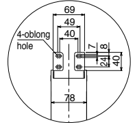
Z-axis cable wiring Detail view of moving end of cable track
