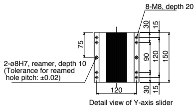
Detail view of Y-axis slider
