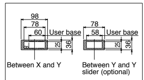
Section view of cable storage space
