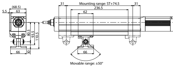
EC-RR6□AH/RR6□AHR Single unit model: EC-QRPB-RR6
