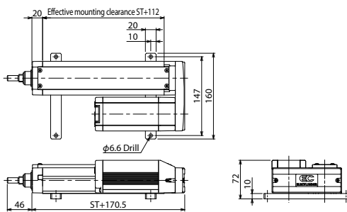
EC-RR6□AHR Single unit model: EC-FT-SRR6R
