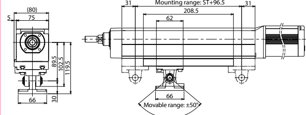
EC-RR7□AH/RR7□AHR Single unit model: EC-QRPB-RR7
