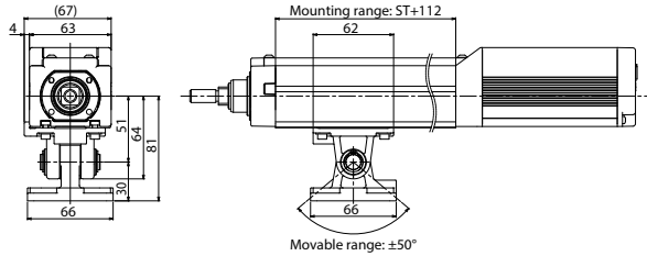
EC-RR6/RR6□R Single unit model: EC-QRPB-RR6
