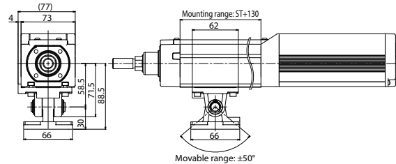
EC-RR7/RR7□R Single unit model: EC-QRPB-RR7
